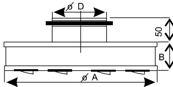
Diffuser ONS/RD, ONS/RDM version 1
