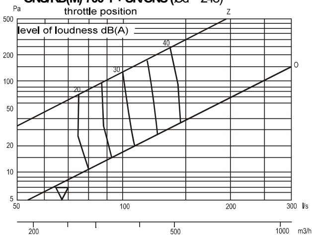
ONS/RD(M) 700-1 + SR/ONS (Ød = 248)
