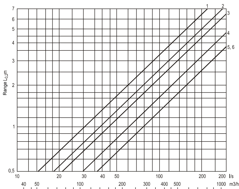
ONS/RD(M) 2 lower nozzles arranged in the opposite direction than the upper
