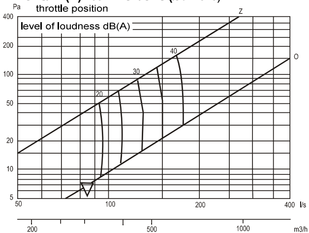
ONS/RD(M) 700-1 + SR/ONS (Ød = 313)
