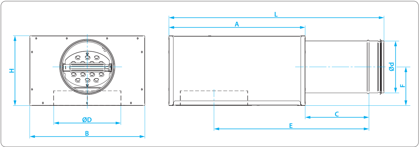
Figure 04 - Dimensions TK - 1-2 step type
