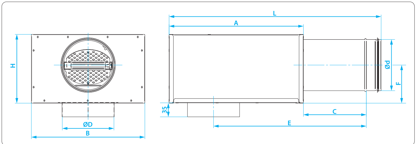
Figure 03 - Dimensions TK - 0-step type
